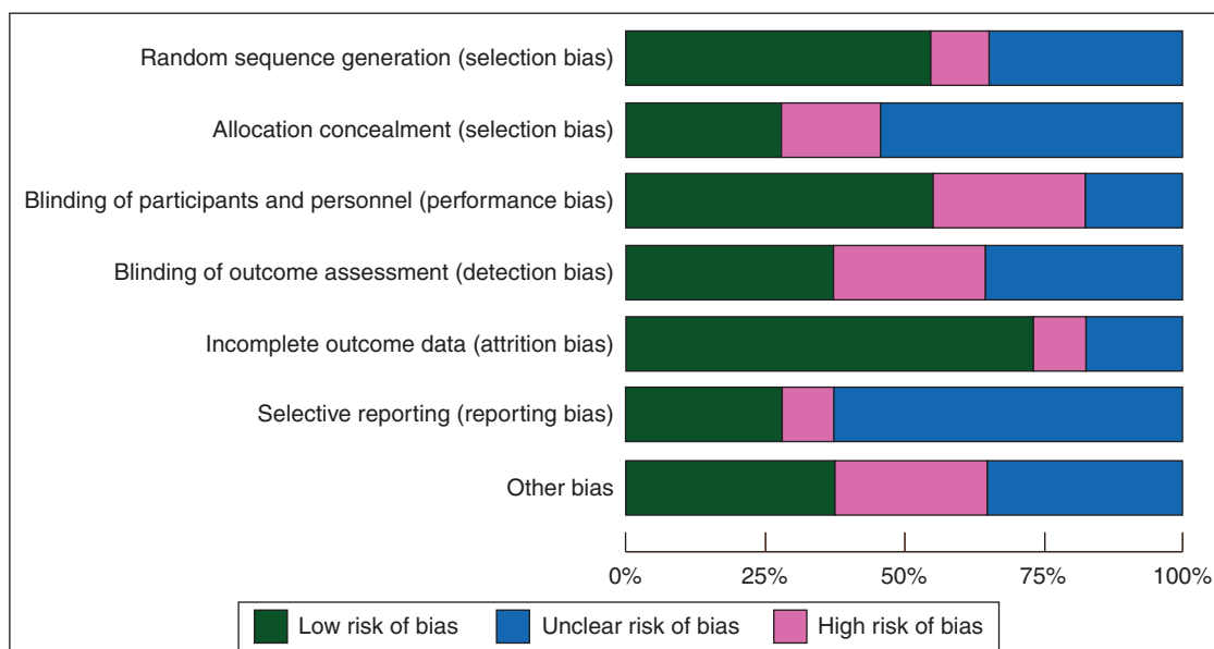
Figure 3. Bar chart comparing percentage risk of bias for each item as judged according to Cochrane 'Risk of bias' assessment tool. Data from [15].
